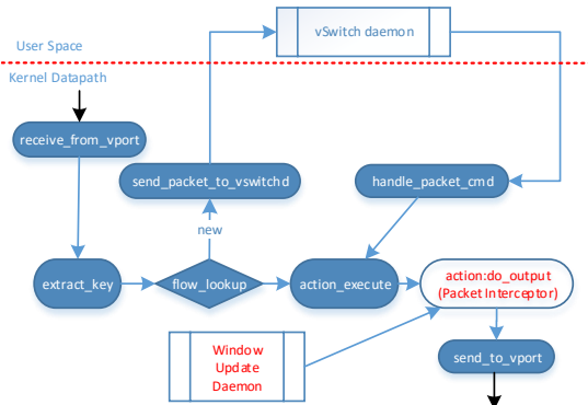
(b) OpenvSwitch-based RWNDQ packet processing pipeline
