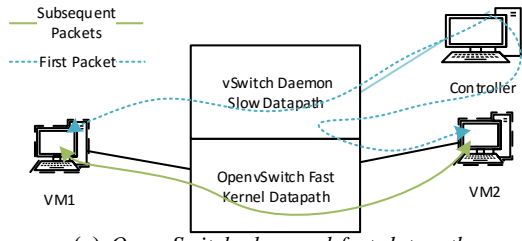
(a) OpenvSwitch slow and fast datapath
