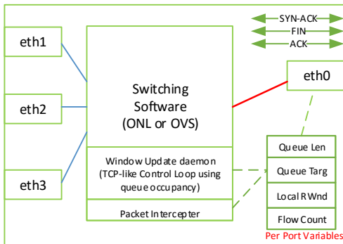
Figure 1: RWNDQ high level system-view design
