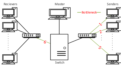
Figure 8: Small testbed for RWNDQ-enabled OvS
